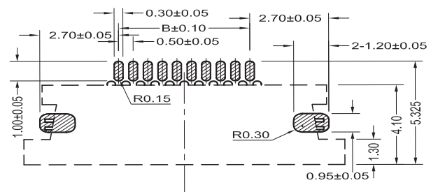
R3 and R4 PCB Layout Reference
